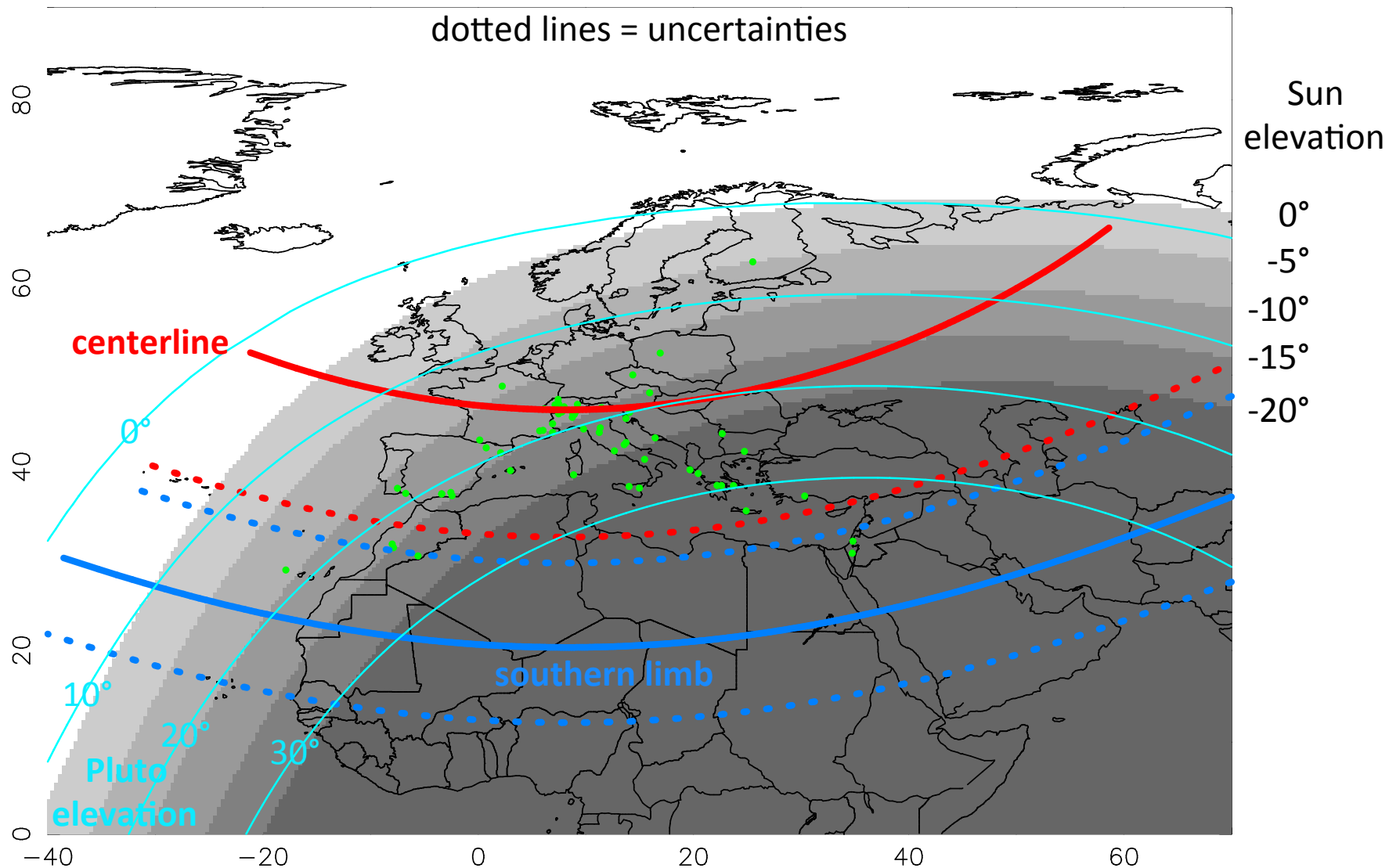
Pluto 19 Jul 2016 (~20:50 UT), red: centerline, blue: southern limit
