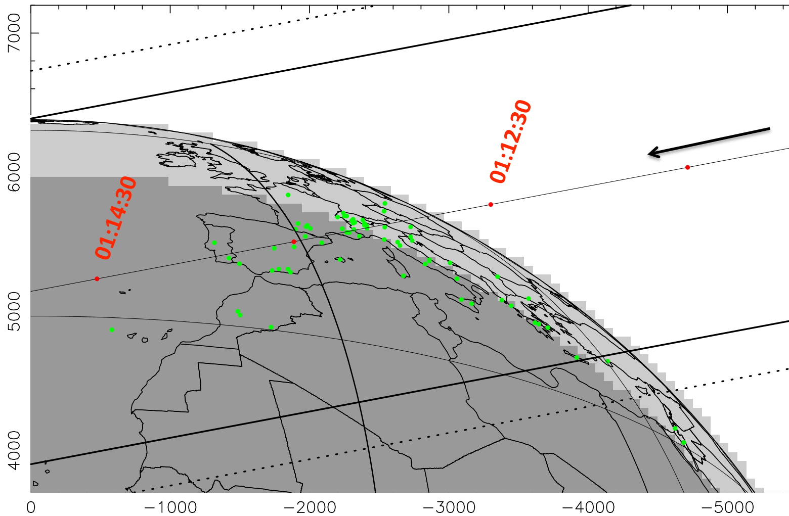
Pluto 14jul16, BS/15jul16 post-occ, offset (+82.53,-28.998) mas
